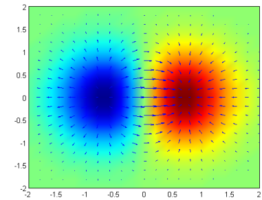
Figure 2: Gradient of the 2D function f(x, y) = xe^{(x^2+y^2)} is plotted as blue arrows over the pseudocolor (red is for high values while blue is for low values) plot of the function. Source .
