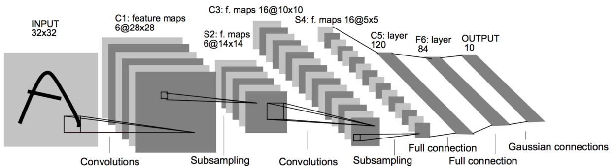
Figure 25: LeNet architecture. Source .
