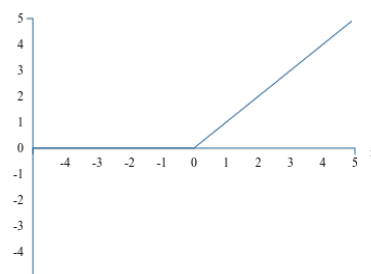
Figure 9: ReLU. Source .
